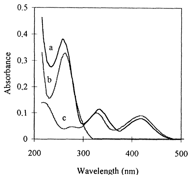
Figure 2. UV spectra of 12* (a), UM (b) and 12 (c).
